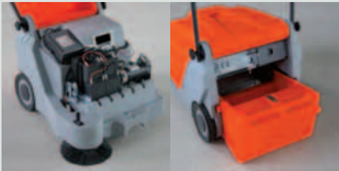
Clearly laid out construction, easy adjustment, maintenance-free battery system. Large 40 l synthetic material dirt hopper.
